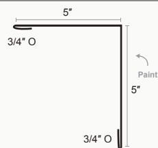
Standing Seam Locking Outside Corner
