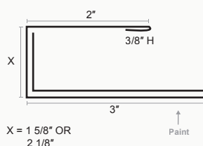
Soffit C Metal Color in
