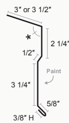
Custom Eave
