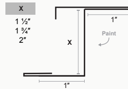
SnapZ
