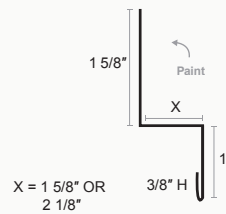
Z Metal Wall Lite
