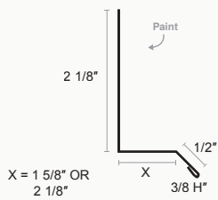
Standing Seam Base Metal
