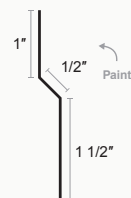
Standing Seam Offset Cleat
