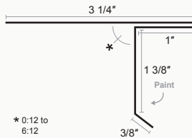
Style D
