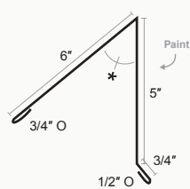
Standing Seam Locking Peak Cap
