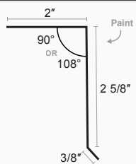
Eave Flashing
