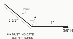
Standing Seam Pitch Break
