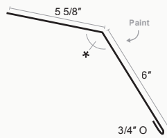
Standing Seam Locking Reverse Pitch Break
