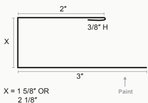
Standing Seam Soffit C Metal
