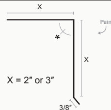
Drip Flashing
