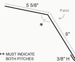
Standing Seam Reverse Pitch Break
