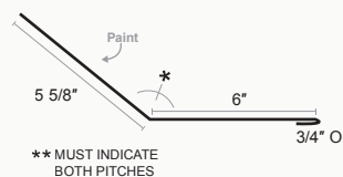
Standing Seam Locking Pitch Break
