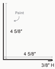
Standing Seam Side Wall
