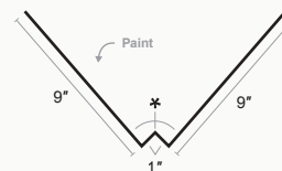
Standing Seam W Valley
