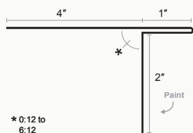
Bull Nose Eave
