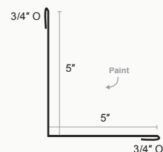
Standing Seam Locking Inside Corner
