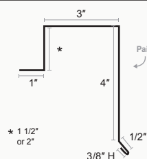
Standing Seam Box Gable
