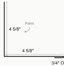
Standing Seam Locking Side Wall
