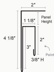
Flush Wall F and J Channel
