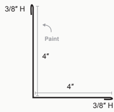
Flush Wall Inside Corner
