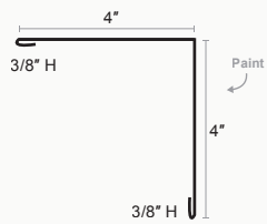
Corrugated Outside Corner
