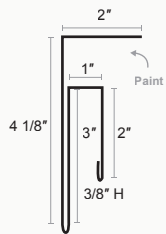
F and J Trim
