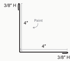
Corrugated Inside Corner
