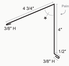
Peak Cap
