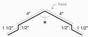
Universal Ridge Cap
