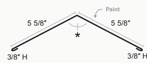
Ridge Cap Low Profile
