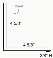
Corrugated Side Wall
