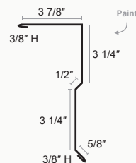
Corrugated Gable Trim
