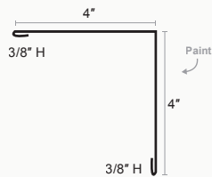
Corrugated Outside Corner
