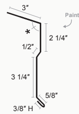
Custom Eave
