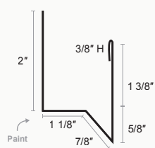
Corrugated Head Trim
