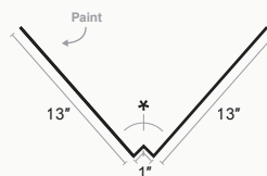
W Valley
