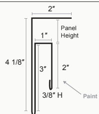
F and J Trim
