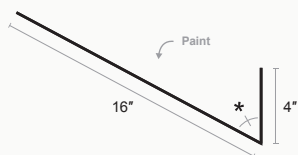
Chimney Flashing
