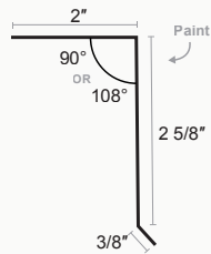
Eave Flashing
