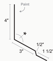
End Wall Flashing
