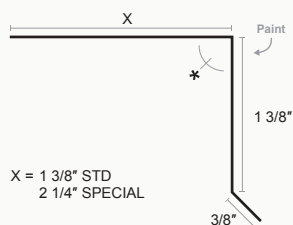
Style G Drip
