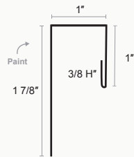
C Metal
