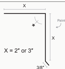
Drip Flashing
