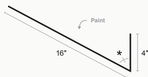
Chimney Flashing
