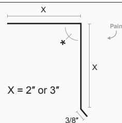
Drip Flashing
