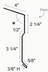
Custom Eave
