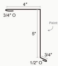
Standing Seam Locking Gable
