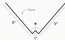
Standing Seam W Valley
