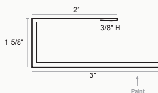
Standing Seam Soffit C Metal 1.5 Color in
