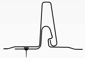
EAVES & END LAPS
