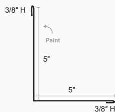
Standing Seam Inside Corner
