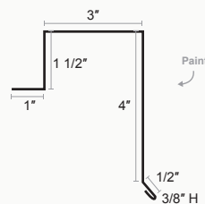
Standing Seam Box Gable 1.5
