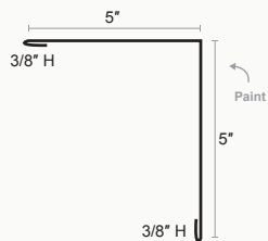
Standing Seam Outside Corner
