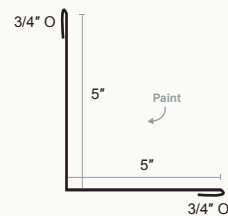
Standing Seam Locking Inside Corner
