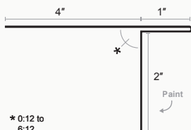
Bull Nose Eave
