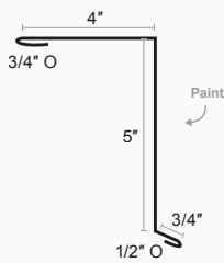
Standing Seam Locking Gable
