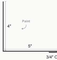
Locking Side Wall Flashing
