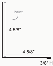
Standing Seam Side Wall
