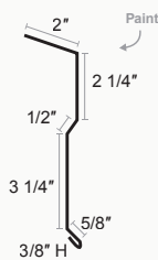
Standing Seam Rake A
