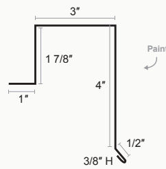
Standing Seam Box Gable_1.75
