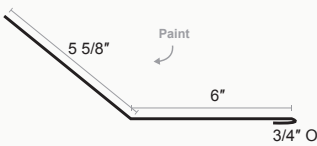
Standing Seam Locking Pitch Break
