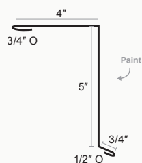
Standing Seam Locking Gable
