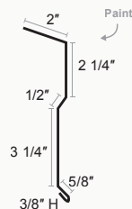
Standing Seam Rake A
