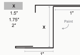
SnapZ Vented Z Bar
