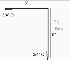
Locking Outside Corner
