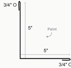
Locking Inside Corner
