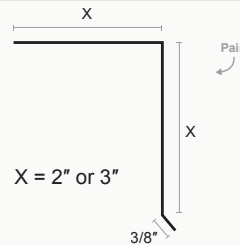
Drip Flashing
