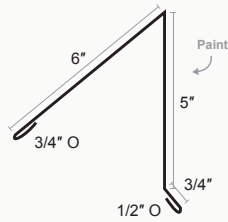
Standing Seam Locking Peak Cap
