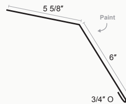
Standing Seam Locking Pitch Break Reverse
