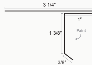
Style D
