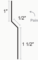
Offset Cleat
