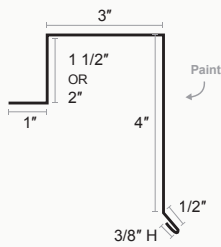
Standing Seam Box Gable
