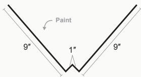
Standing Seam Ridge Valley
