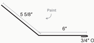
Standing Seam Locking Pitch Break
