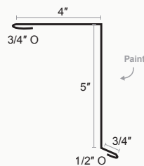
Standing Seam Locking Gable
