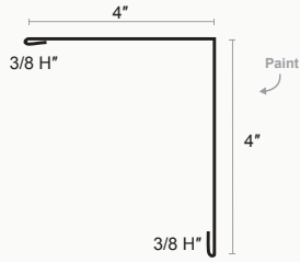
B_B Outside Corner
