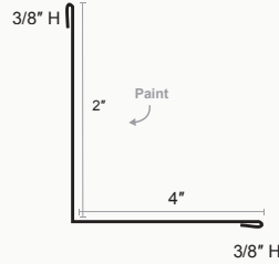
B_B Inside Corner
