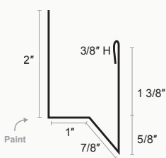
B_B Head Trim
