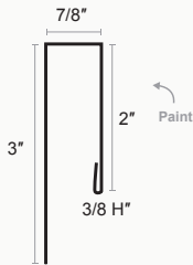
B_B C Metal
