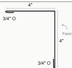
B_B Locking Outside Corner
